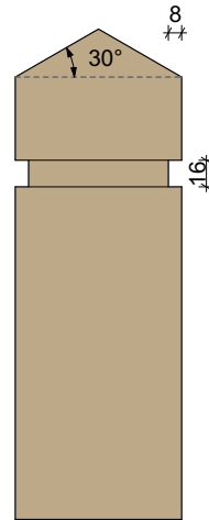
Pyramid Top With Rebated Collar (x1)
