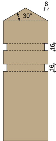
Pyramid Top With Rebated Collar (x2)
